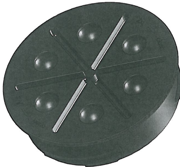
Figure 1: sealing cover HSI 150-D (Manufacturer drawing)
